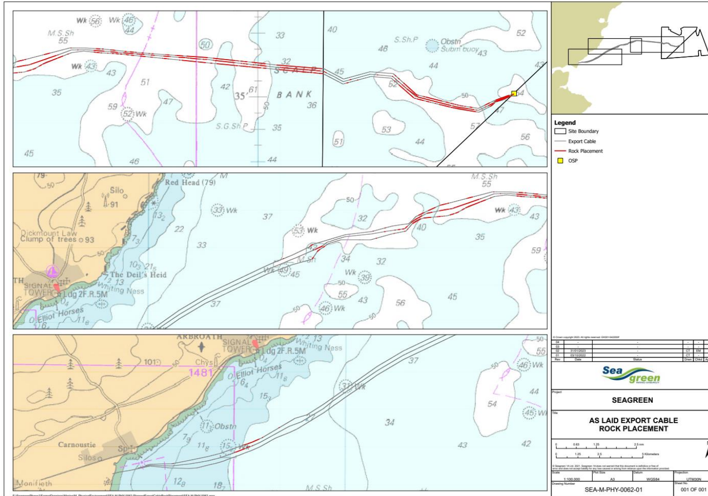
2. Figure 1 – Rock placement locations
