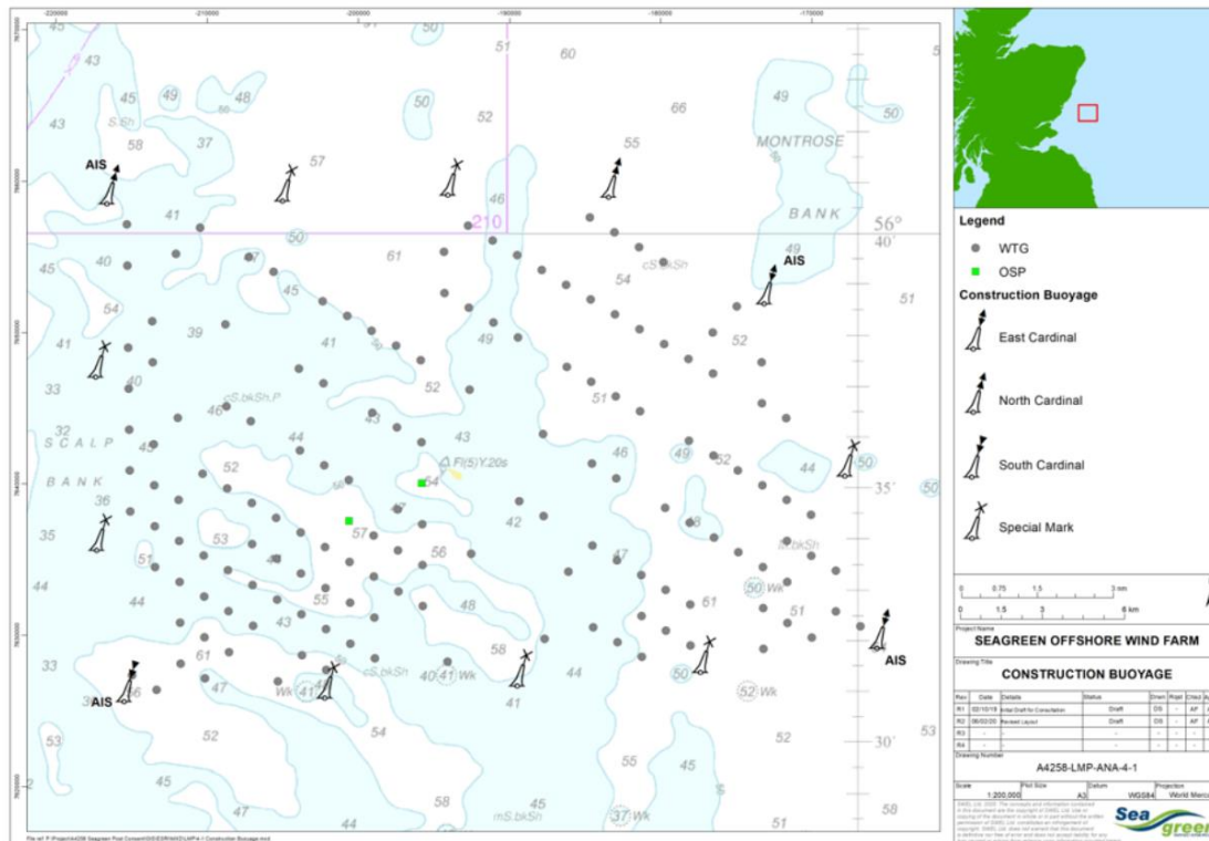
Fig 1 – Demarcation buoy location
