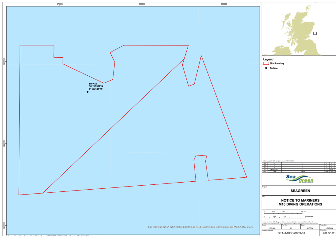
Fig 1 – SN-M10 WTG foundation location.
