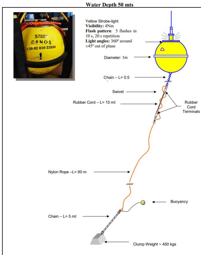
Fig 2 – Buoy mooring arrangement and lighting characteristics.
