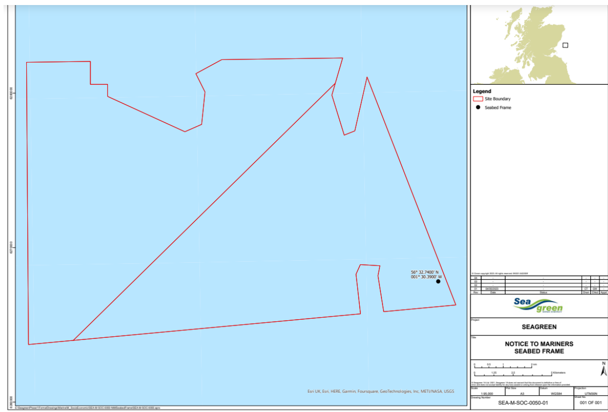
Fig 1 – Seabed frame locations and coordinates.
