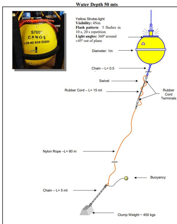
Fig 2 – Buoy mooring arrangement and lighting characteristics.
