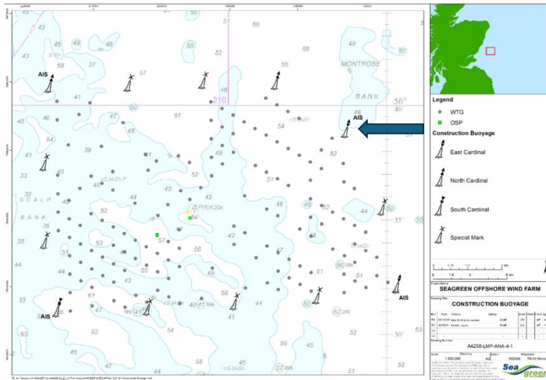
Fig 1 – Buoy as-laid position as shown by blue arrow.
