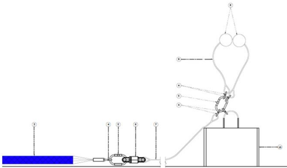
Fig 3 – Cable end mooring arrangement
