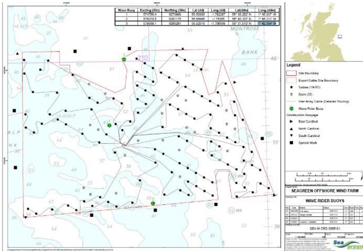
Fig 1 – Demarcation and wave data buoy location.
